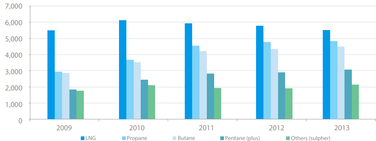
Chart 4: Production of Liquefied Natural Gas Products*
