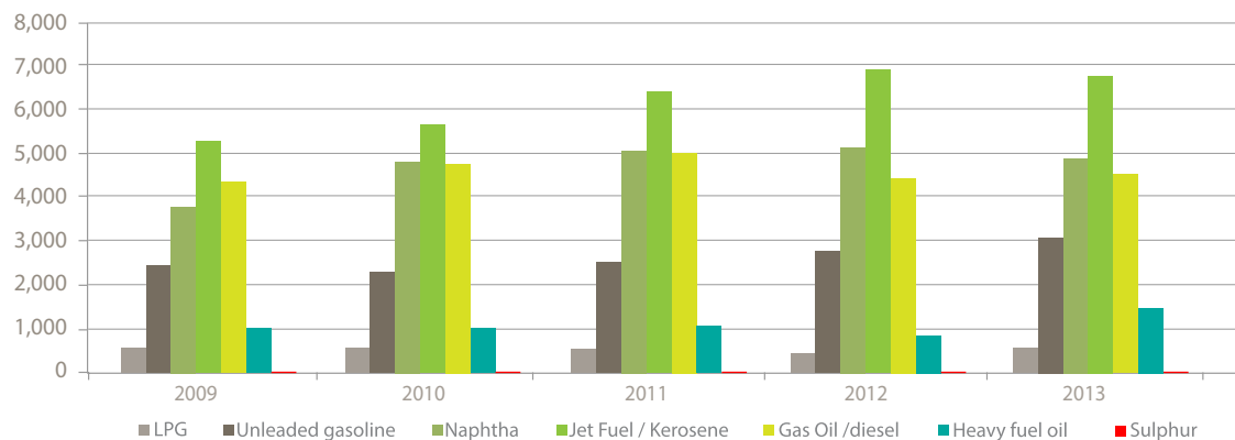
Chart 2: Production of refined petroleum products Thousand Metric Tons
