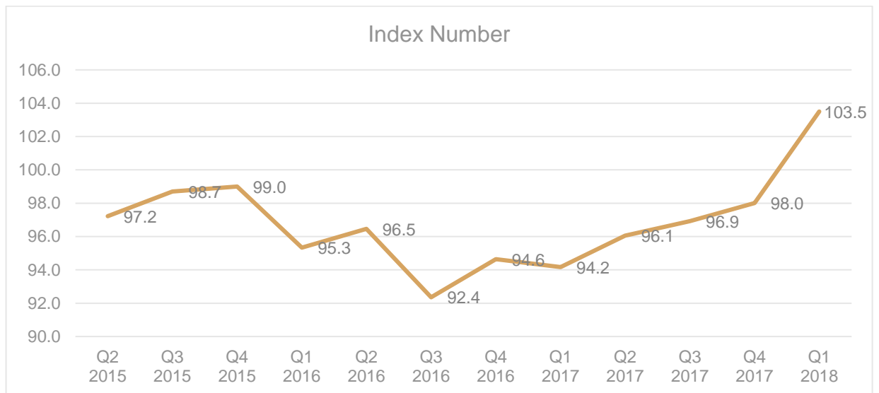
Figure 1: Construction Cost Index, quarterly for 2015, 2016, 2017 and 2018 (2013=100)
