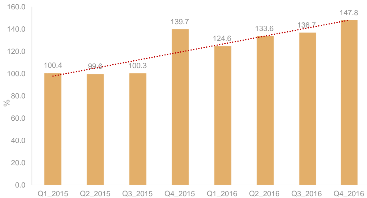
Figure 1: Quarterly Industrial Production Index (IPI) for 2015, 2016 (2012=100)
