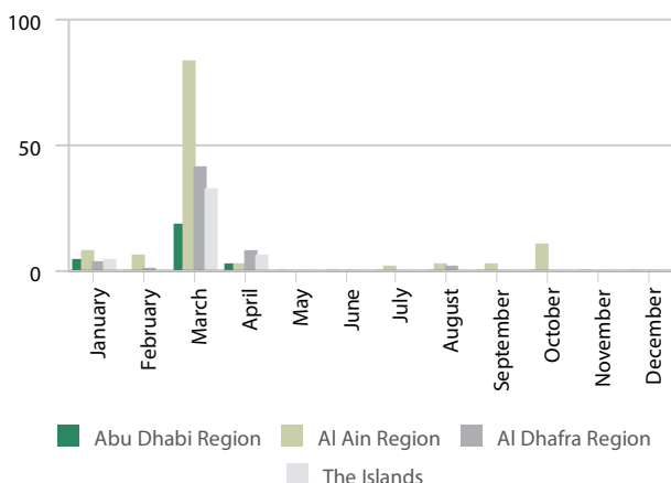
Figure 6.2.3 Average Rainfall by Month and Region, 2016
