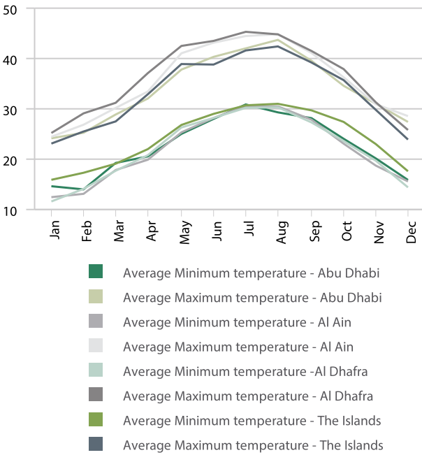
Figure 6.2.2 Average maximum and minimum air temperature by month and region, 2016
