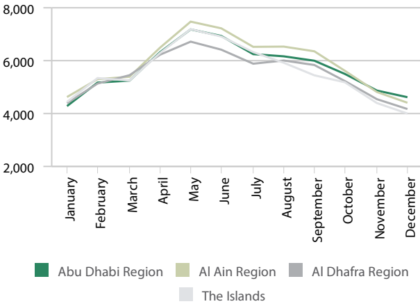
Figure 6.2.5 Average Daily Total Solar Radiation by Month and Region, 2016
