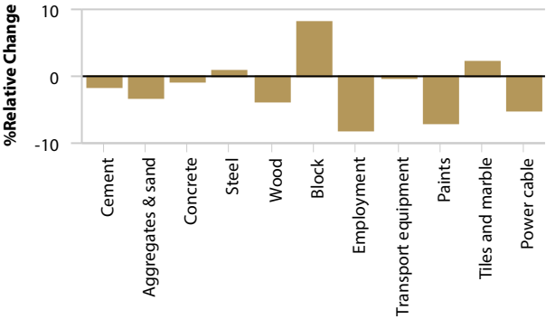
Figure 1.3.7 Relative Change in Price Averages of the Main Groups of Building Materials in 2016 Compared with 2015
