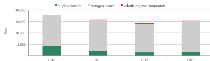
Figure 6.2.7. Air Pollutant Total Emissions - Water and Electricity Production Sector
